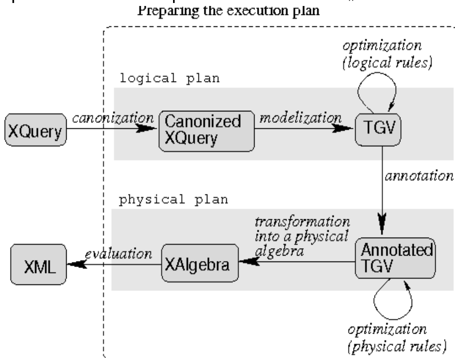
#Figure 2: XQuery Evaluation Process##
